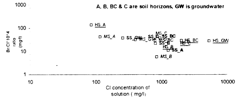
Figure 2. The ratio of bromide to chloride in the saturation extracts of soil genetical horizons and groundwater samples of the three profiles (MS=Mollic Solonetz, SS=Salic Solonetz and HS=Haplic Solonetz).
