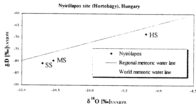
Figure 4. The \delta\text{D} vs. \delta^{18}\text{O} values of three observation wells in the Nyirólapos (Hortobágy, Hungary) area in the year 1998.
